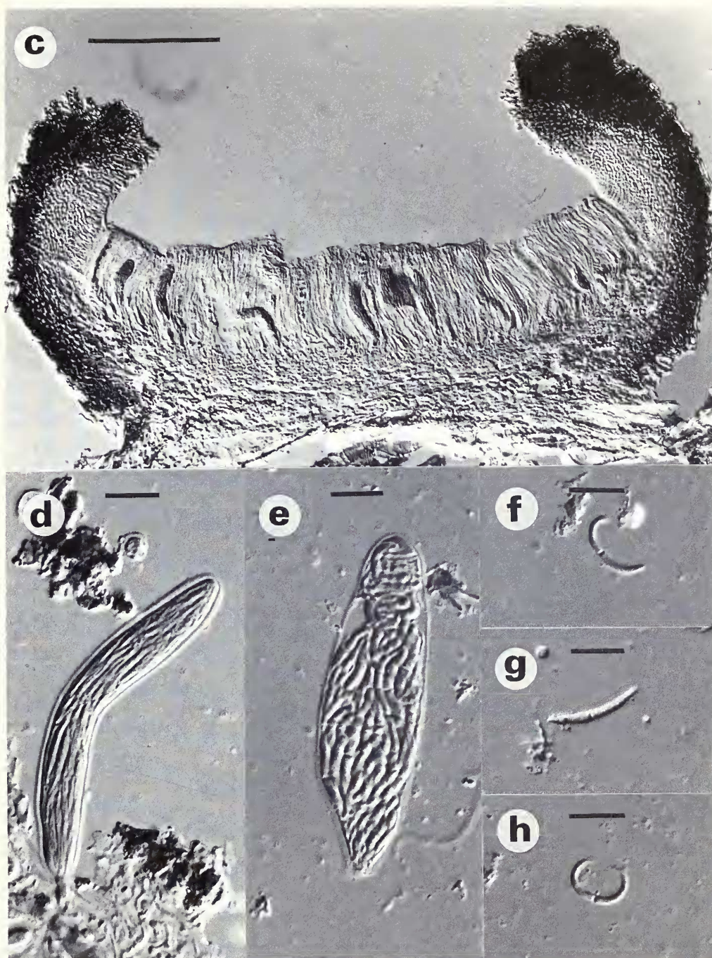
Fig. 72 Odontura rhapsidospora (Rehm) Clem. (S-lectotype) (c) Vertical section of ascoma, showing marginal layer of periphysoids; scale = 100 \mu\text{m} ; (d) Ascus and ascospores; (e) Ascus and part-ascospores; (f), (g), (h) Part-ascospores; scale = 10 \mu\text{m} .
